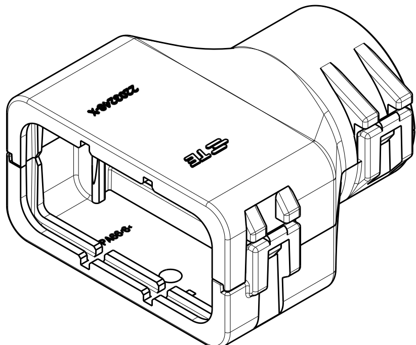
2292865-3 ASSEMBLED ISOMETRIC VIEW SHOWN
