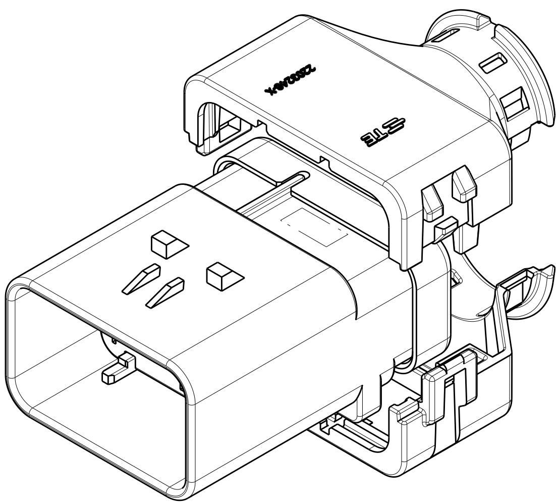
2292865-1 WITH CAP ASSEMBLY 2292865-2 EXPLODED ISOMETRIC VIEW SHOWN
