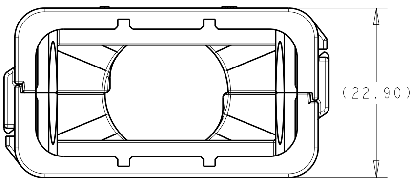
2292865-1 ASSEMBLED VIEW SHOWN
