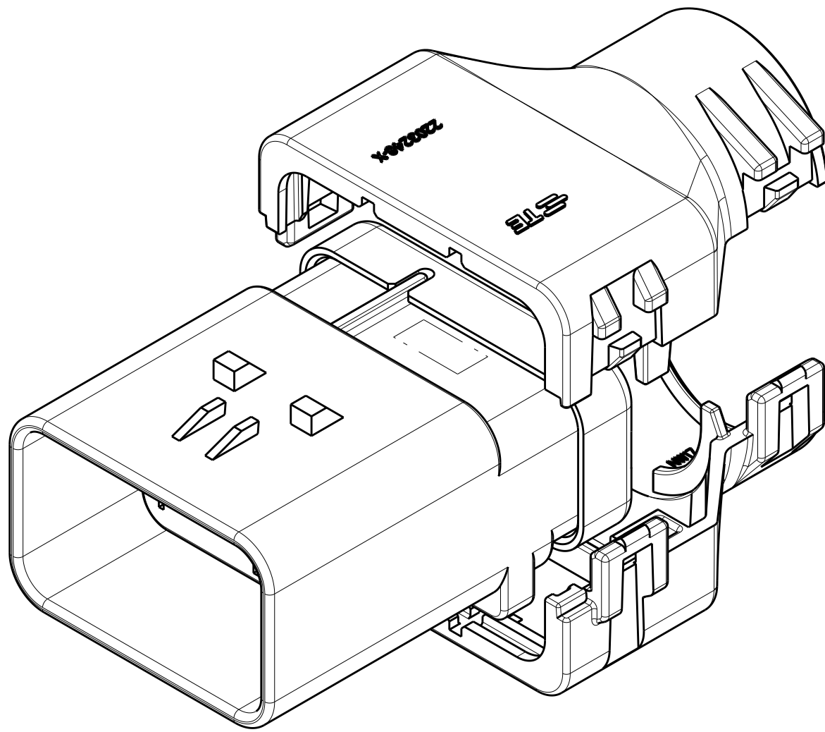
2292865-2 WITH CAP ASSEMBLY 2292865-3 EXPLODED ISOMETRIC VIEW SHOWN
