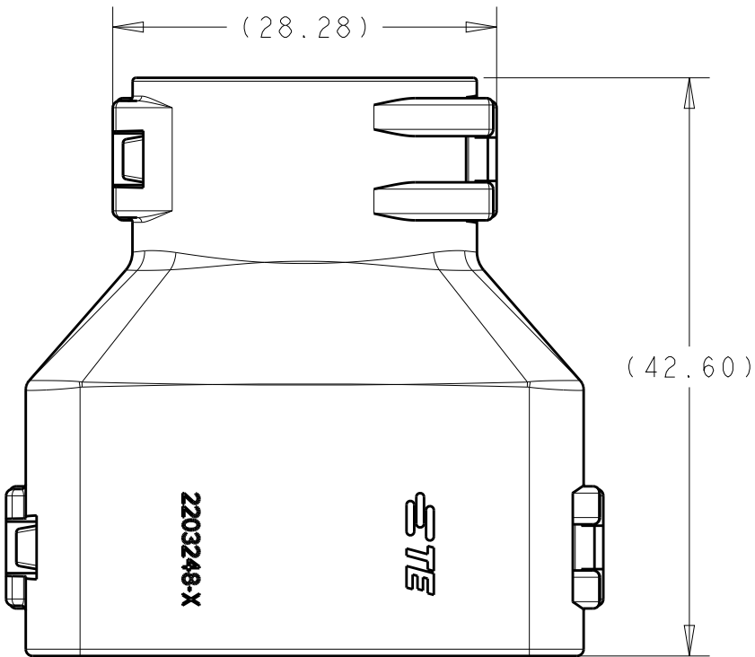
2292865-2 ASSEMBLED VIEW SHOWN
