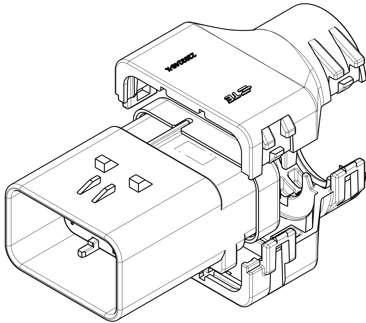
2292865-3 WITH CAP ASSEMBLY 2292865-4 EXPLODED ISOMETRIC VIEW SHOWN
