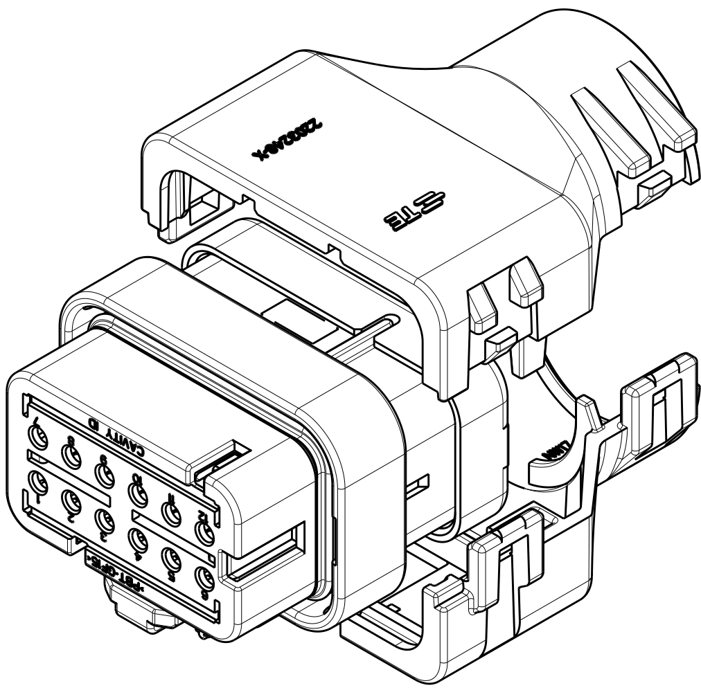
2292802-2 WITH PLUG ASSEMBLY EXPLODED ISOMETRIC VIEW SHOWN
