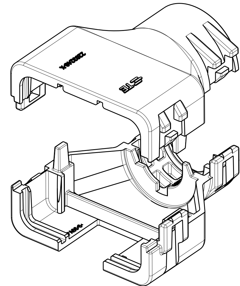
2292802-3 EXPLODED ISOMETRIC VIEW SHOWN
