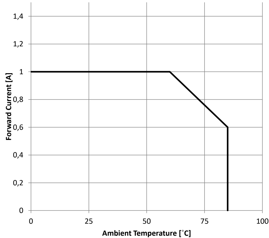
Derating Curve:
