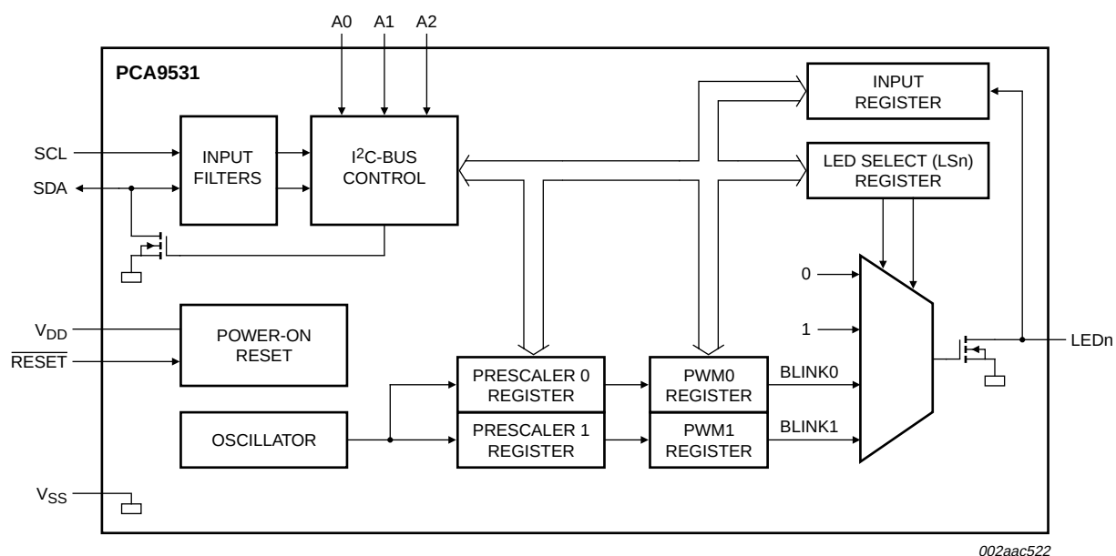
Fig 1. Block diagram of PCA9531
