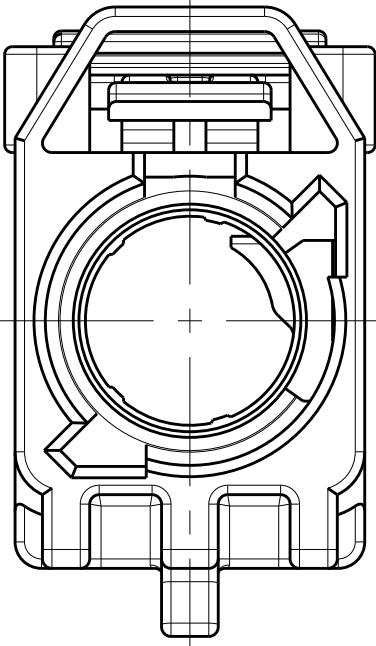
DETAIL N SCALE 5:1
