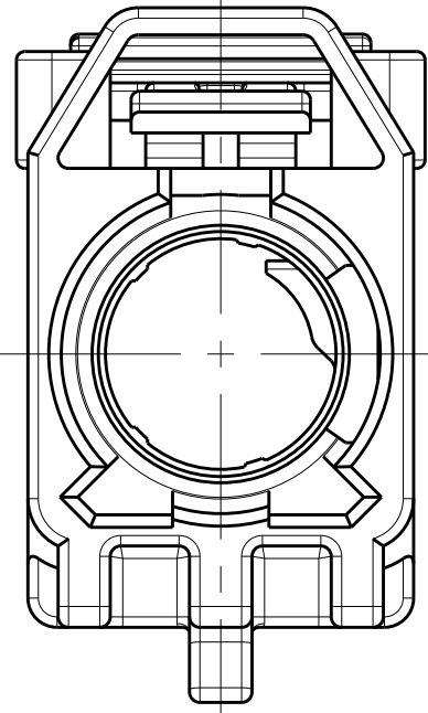
DETAIL L SCALE 5:1
