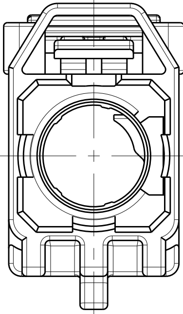
DETAIL Z SCALE 5:1
