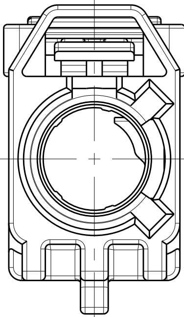
DETAIL D SCALE 5:1
