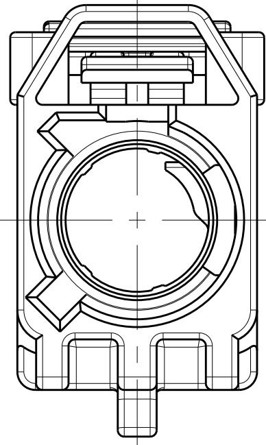
DETAIL F SCALE 5:1
