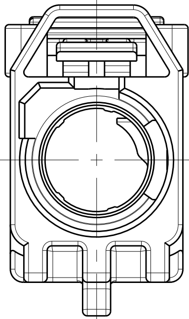
DETAIL E SCALE 5:1
