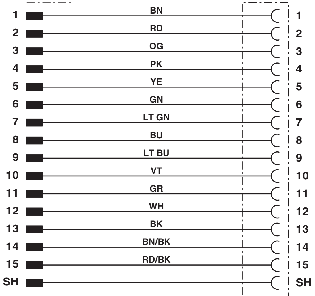
Circuit diagram
