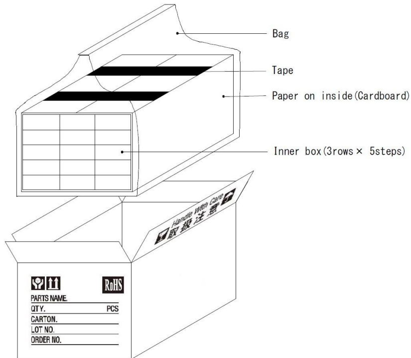
Figure 11 – Outer-Box Packaging
