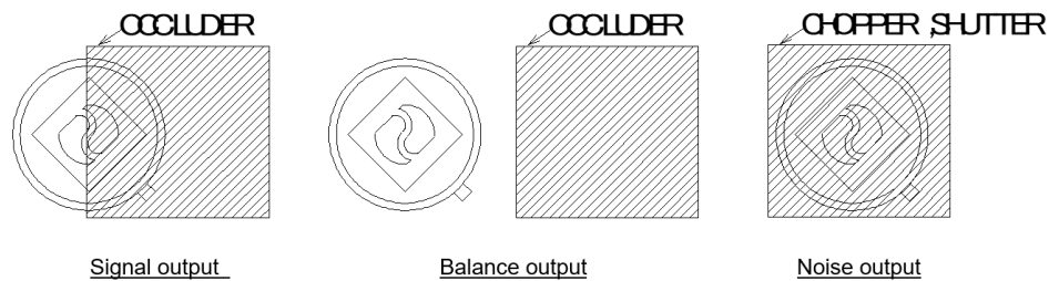
Figure 2 - Occluder Position
