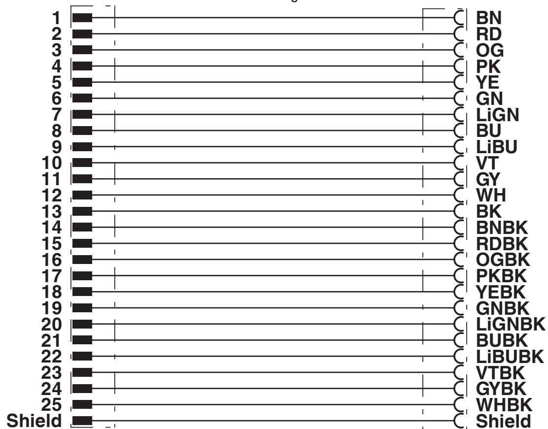
Circuit diagram
