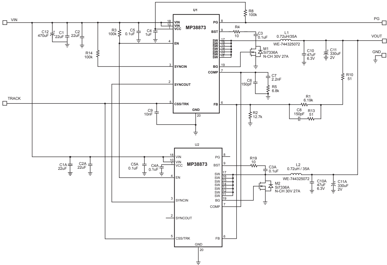
Figure 7—Two Phase Operation
