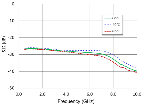
Reverse Isolation
