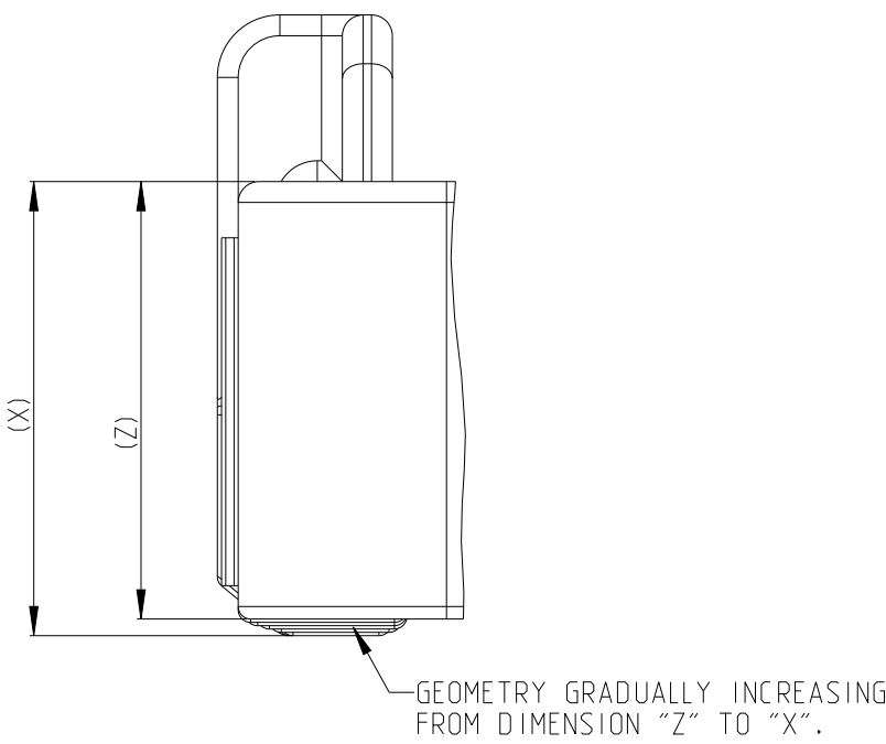
DETAIL Z SCALE 5:1
