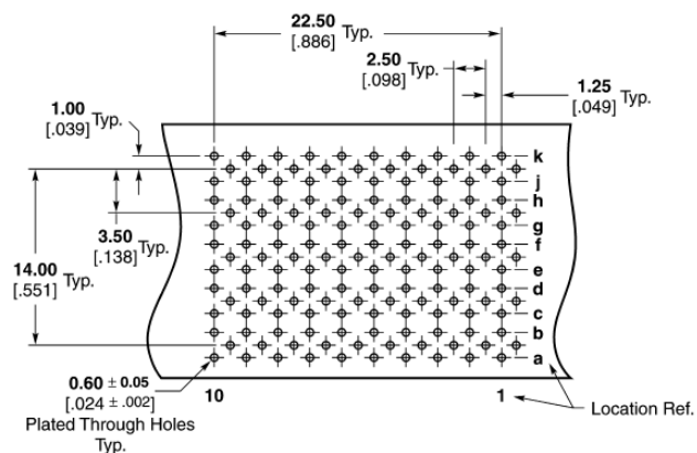
Non-Coplanar Daughtercards (Pin 1a Header = Pin 1k Shroud Side) Recommended PC Board Layout — Reference Page 126 (Shroud Side Shown)
