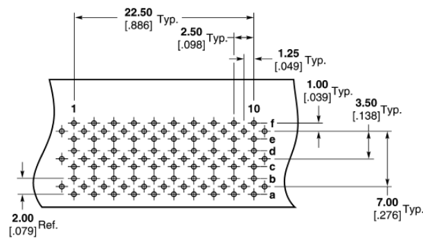
Coplanar Daughtercards (Pin 1a Header = Pin 5a Shroud Side) Recommended PC Board Layout — Reference Page 112 (Shroud Side Shown)
