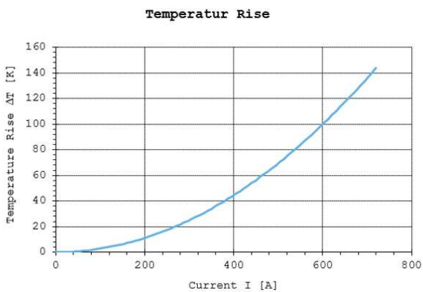
Figure22: Temperature rise without shield current –Header 180deg 2pos +120mm 2 H+S-Part-No. 84103410.
