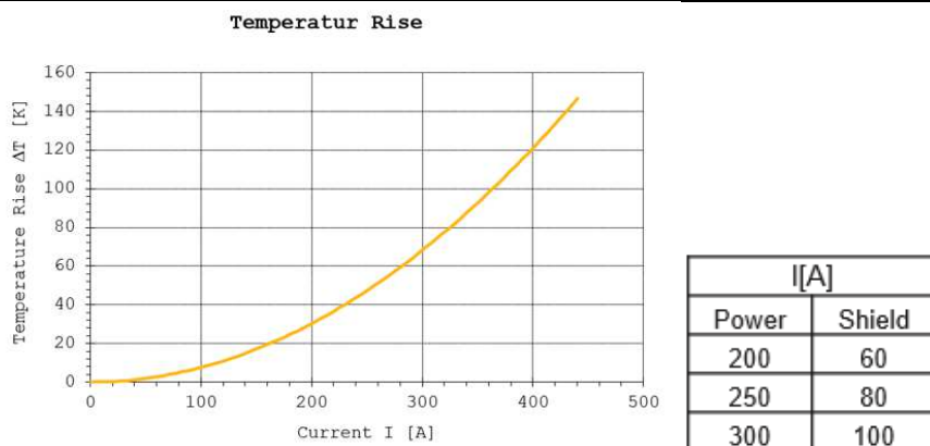
Figure9: Temperature rise with high shield current –Header 180deg 3pos +70mm 2 H+S-Part-No. 84100298.
