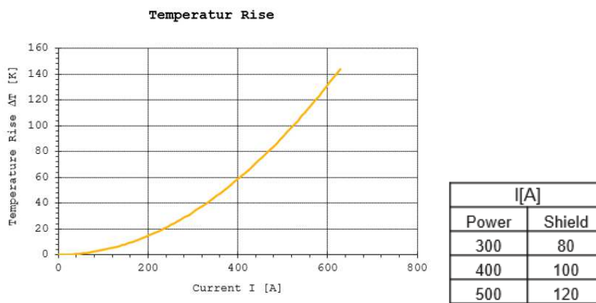
Figure21: Temperature rise with high shield current –Header 180deg 1pos +120mm 2 H+S-Part-No. 84103410.
