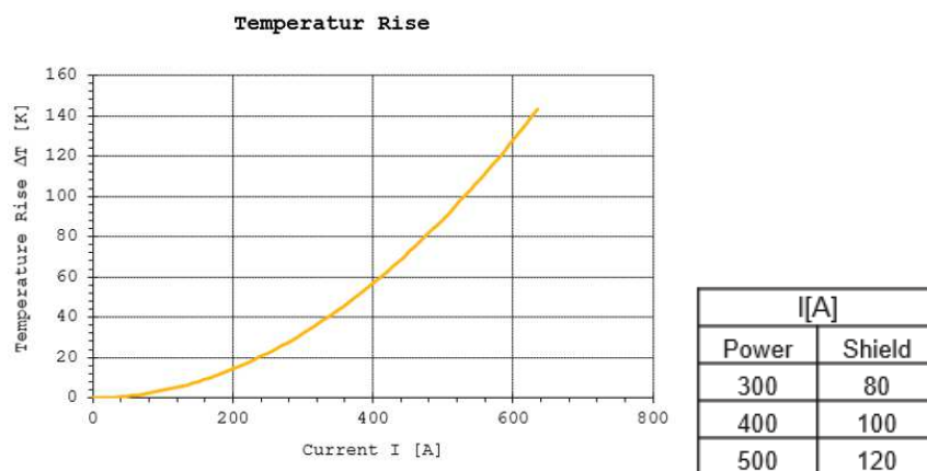
Figure24: Temperature rise with high shield current –Header 180deg 2pos +120mm 2 H+S-Part-No. 84103410.
