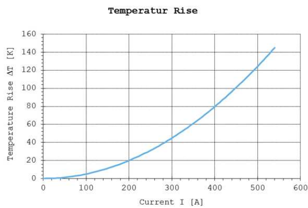
Figure7: Temperature rise without shield current –Header 180deg 3pos +70mm 2 H+S-Part-No. 84100298.
