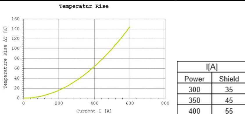
Figure17: Temperature rise with low shield current –Header 180deg 3pos +95mm 2 H+S-Part-No. 84100299.
