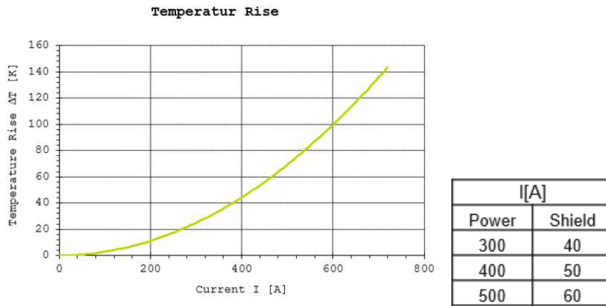
Figure20: Temperature rise with low shield current –Header 180deg 1pos +120mm 2 H+S-Part-No. 84103410.
