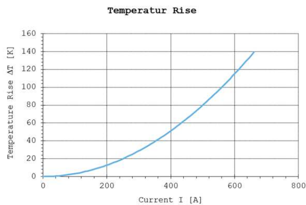
Figure13: Temperature rise without shield current –Header 180deg 2pos +95mm 2 H+S-Part-No. 84100299.
