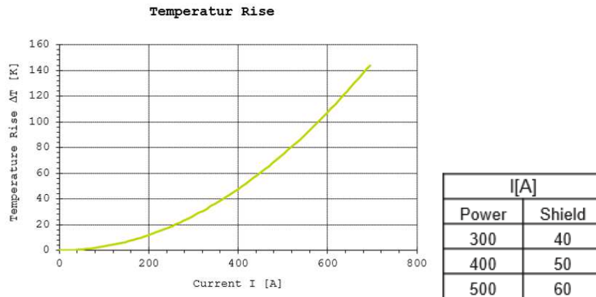
Figure23: Temperature rise with low shield current –Header 180deg 2pos +120mm 2 H+S-Part-No. 84103410.
