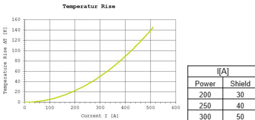
Figure5: Temperature rise with low shield current –Header 180deg 2pos +70mm 2 H+S-Part-No. 84100298.
