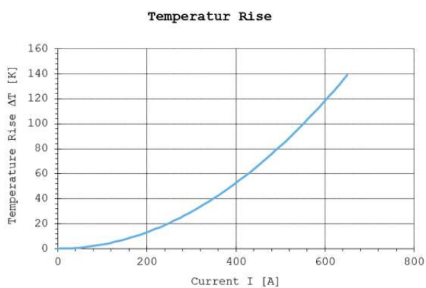
Figure16: Temperature rise without shield current –Header 180deg 3pos +95mm 2 H+S-Part-No. 84100299.
