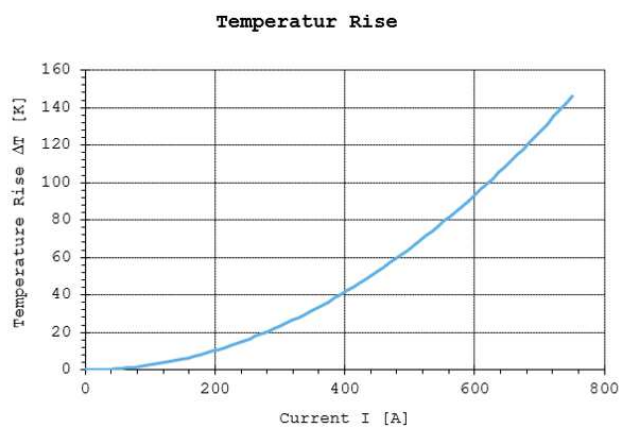
Figure25: Temperature rise without shield current –Header 180deg 3pos +120mm 2 H+S-Part-No. 84103410.
