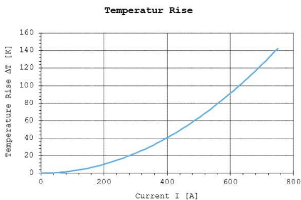
Figure19: Temperature rise without shield current –Header 180deg 1pos +120mm 2 H+S-Part-No. 84103410.
