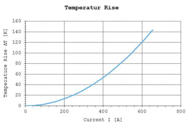
Figure10: Temperature rise without shield current –Header 180deg 1pos +95mm 2 H+S-Part-No. 84100299.
