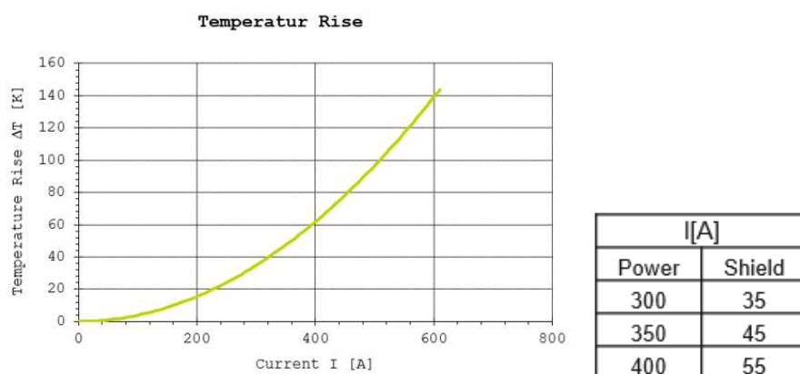
Figure11: Temperature rise with low shield current –Header 180deg 1pos +95mm 2 H+S-Part-No. 84100299.
