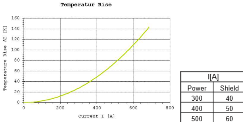
Figure26: Temperature rise with low shield current –Header 180deg 3pos +120mm 2 H+S-Part-No. 84103410.
