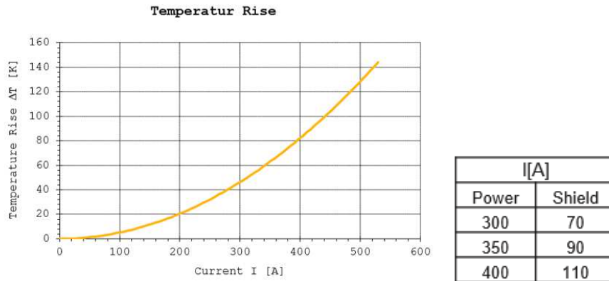
Figure12: Temperature rise with high shield current –Header 180deg 1pos +95mm 2 H+S-Part-No. 84100299.
