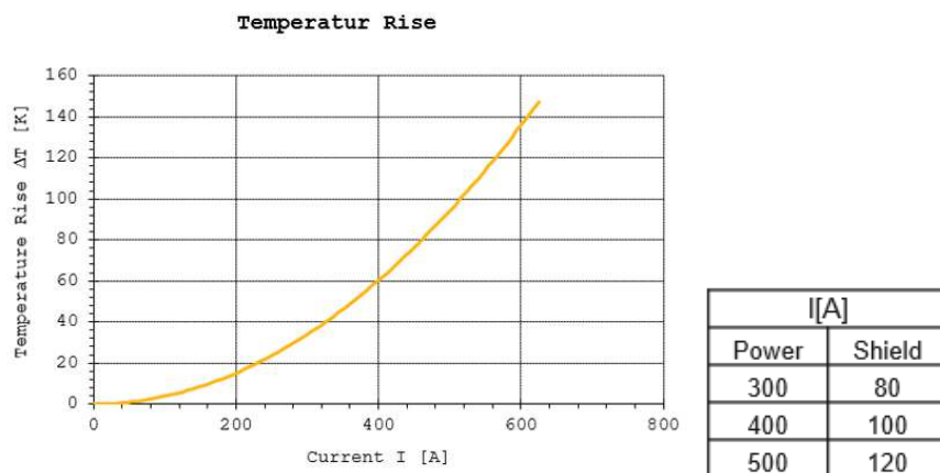
Figure27: Temperature rise with high shield current –Header 180deg 3pos +120mm 2 H+S-Part-No. 84103410.
