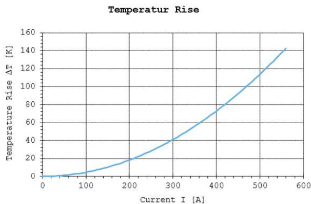
Figure1: Temperature rise without shield current –Header 180deg 1pos +70mm 2 H+S-Part-No. 84100298.
