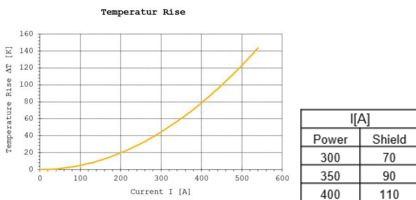
Figure18: Temperature rise with high shield current –Header 180deg 3pos +95mm 2 H+S-Part-No. 84100299.
