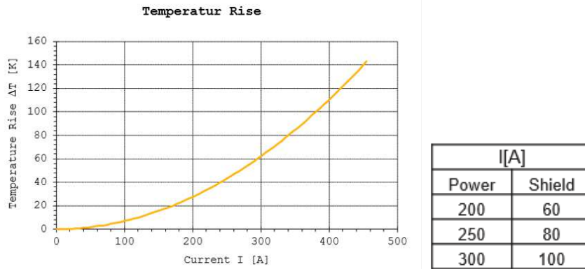
Figure3: Temperature rise with high shield current –Header 180deg 1pos +70mm 2 H+S-Part-No. 84100298.
