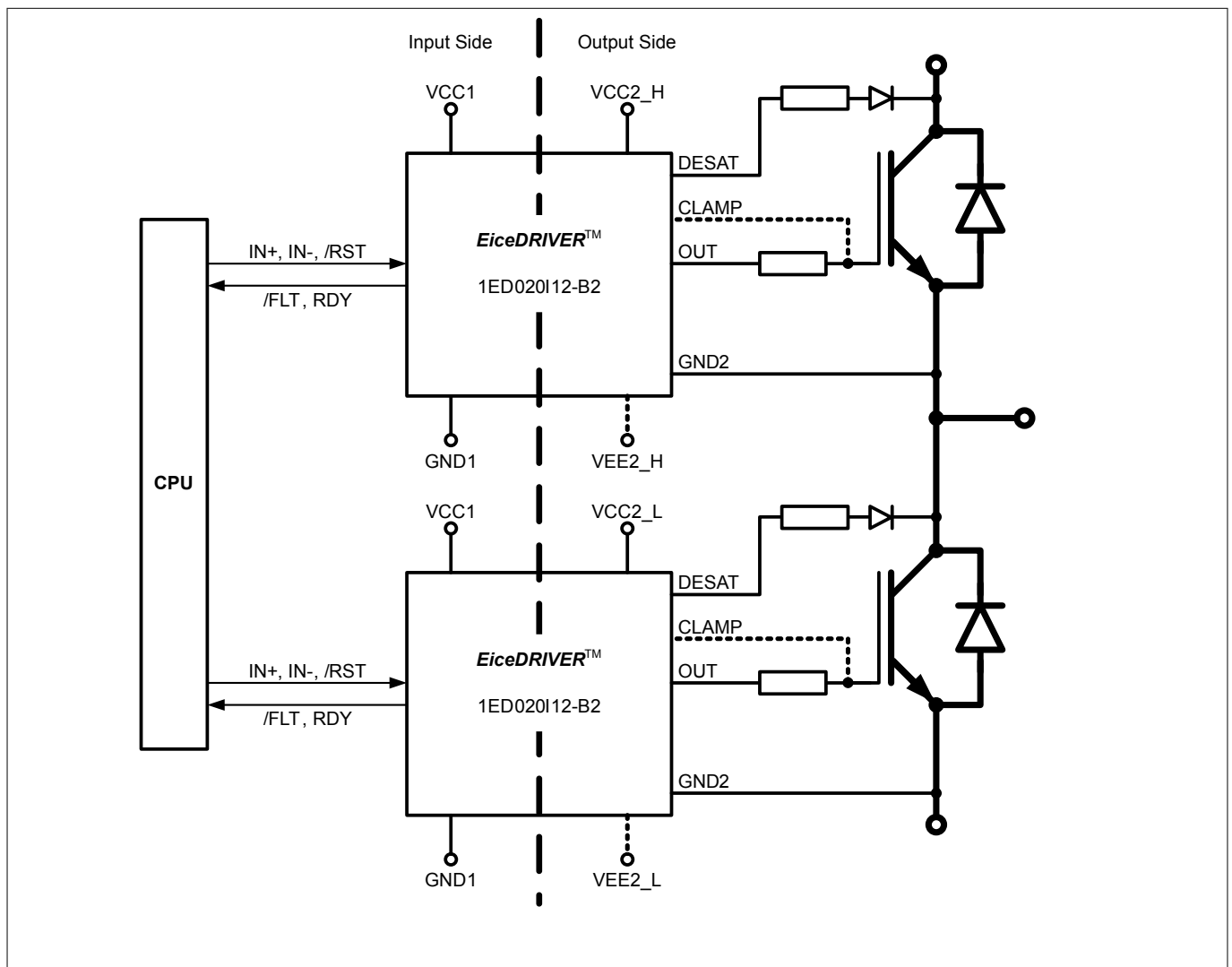
Figure 1 Typical application
